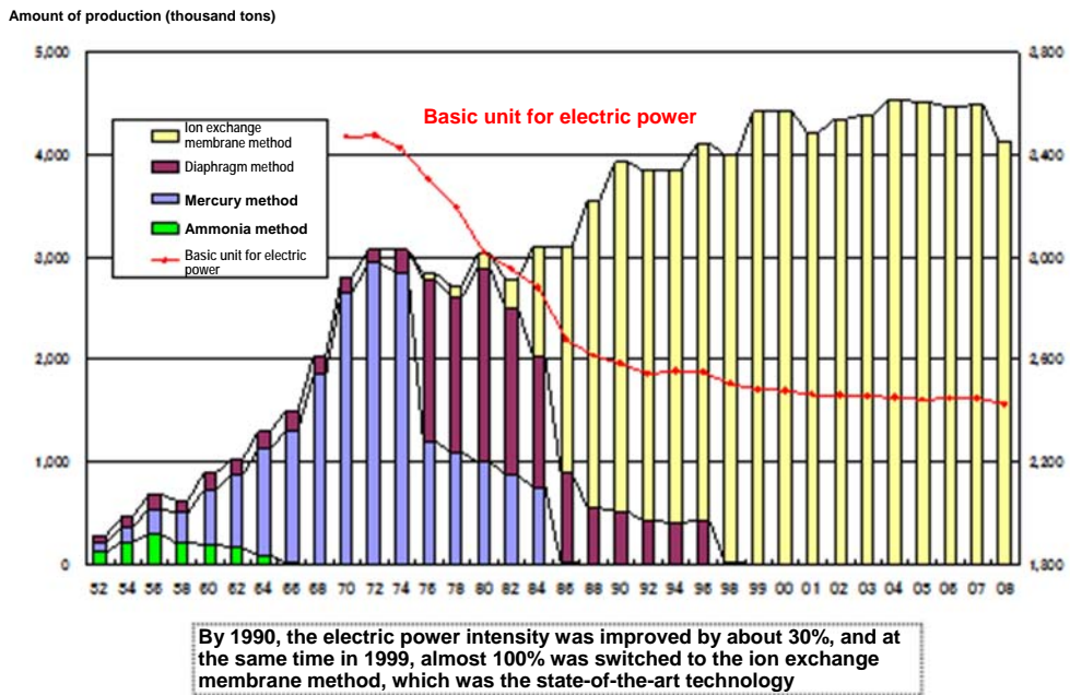
Fig. 11. Changes in energy intensity in the manufacturing processes of ethylene and caustic soda in Japan
