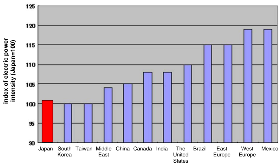
Fig. 14. Comparison of energy efficiency for caustic soda among various countries (electric power intensity for electrolysis, FY2004)
